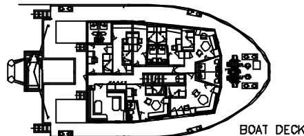
BOAT DECK
