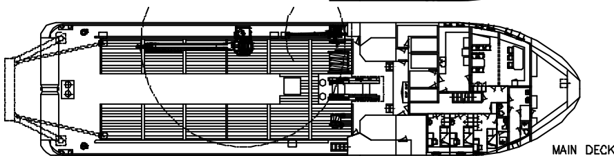
MAIN DECK
